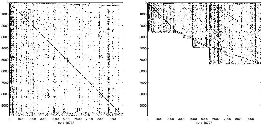
Figure 1: Original \mathbf{P} (left) and reordered \mathbf{P} matrix (right) for CA.dat
